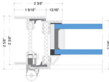
PLANT VIEW ▼
