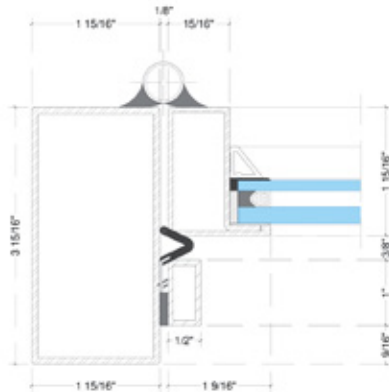
PLANT VIEW ▼
